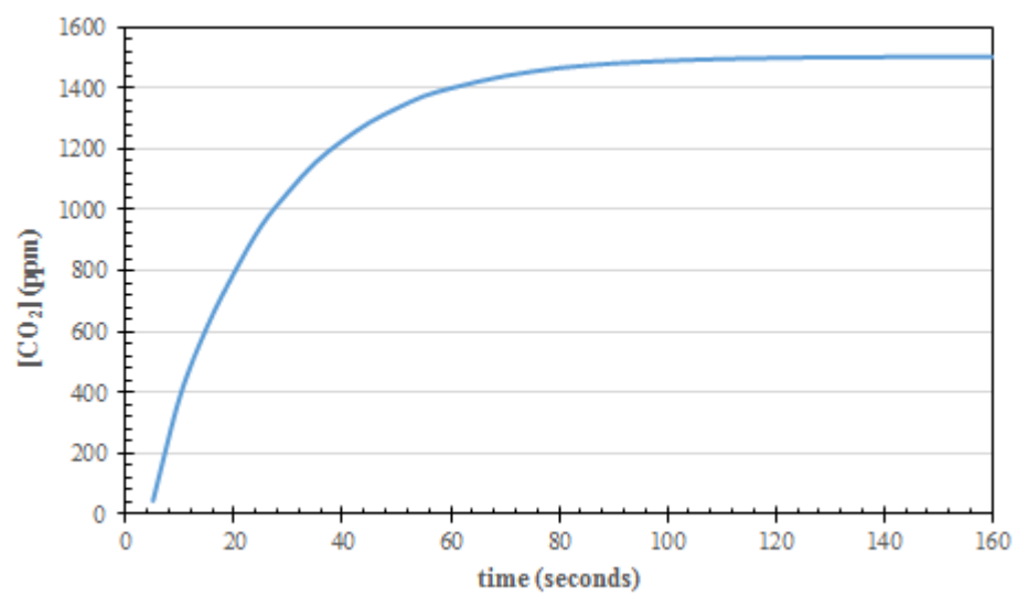
Figure 11. Soil CO 2 Concentrations at VWC = 31.3%.
