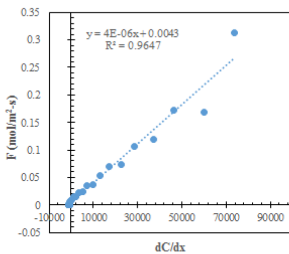
Figure 27. Soil CO 2 flux versus concentration gradient; VWC = 7.8%, replicate 6.
