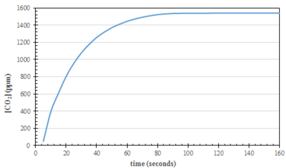
Figure 9. Soil CO 2 concentrations at VWC = 7.8%.
