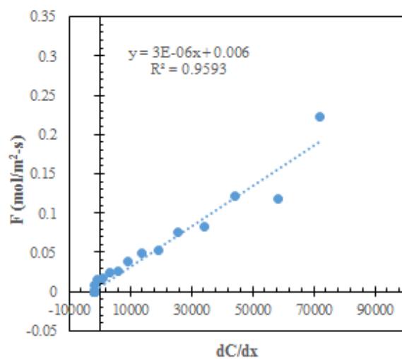
Figure 39. Soil CO 2 flux versus concentration gradient; VWC = 20.5%, replicate 8.
