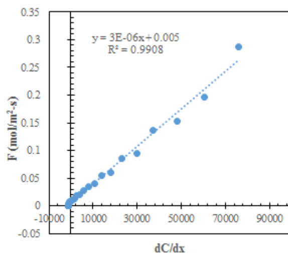
Figure 29. Soil CO 2 flux versus concentration gradient; VWC = 7.8%, replicate 8.
