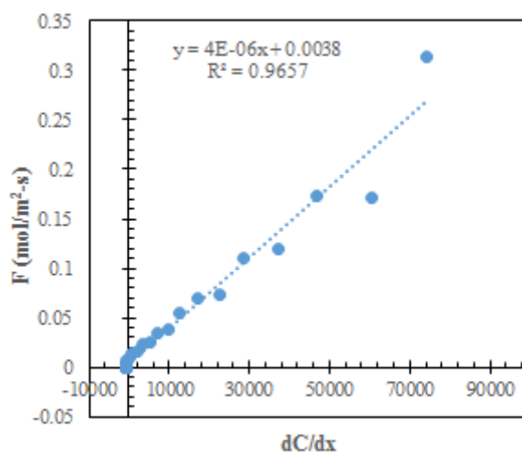
Figure 25. Soil CO 2 flux versus concentration gradient; VWC = 7.8%, replicate 4.
