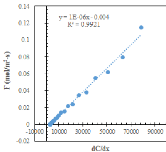
Figure 45. Soil CO 2 flux versus concentration gradient; VWC = 31.3%, replicate 4.
