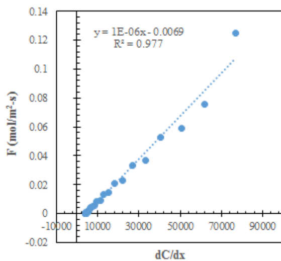
Figure 47. Soil CO 2 flux versus concentration gradient; VWC = 31.3%, replicate 6.
