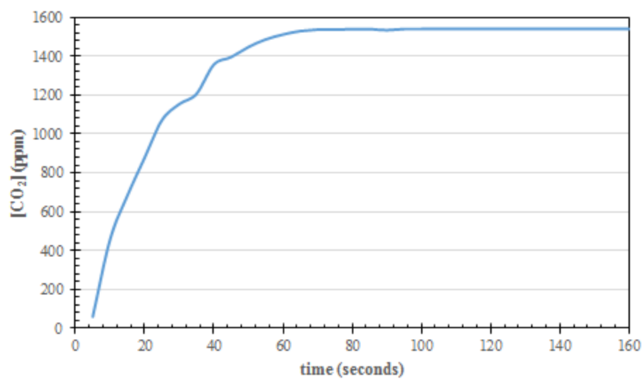
Figure 10. Soil CO 2 concentrations at VWC = 20.5%.
