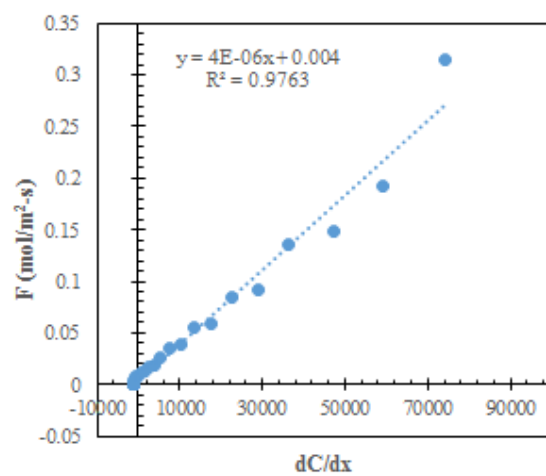
Figure 29. Soil CO 2 flux versus concentration gradient; VWC = 7.8%, replicate 8.
