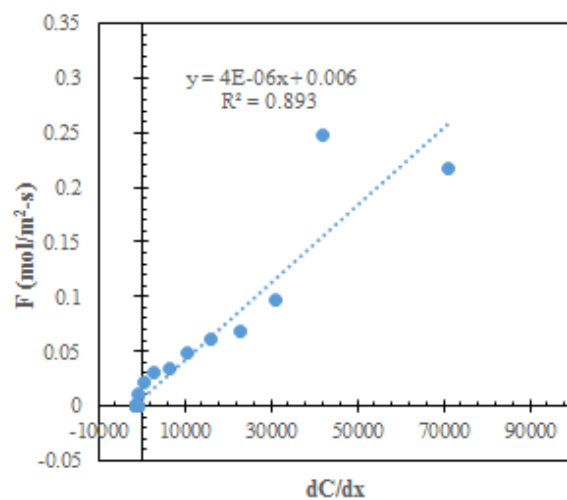
Figure 35. Soil CO 2 flux versus concentration gradient; VWC = 20.5%, replicate 4.
