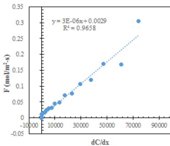
Figure 23. Soil CO 2 flux versus concentration gradient; VWC = 7.8%, replicate 2.
