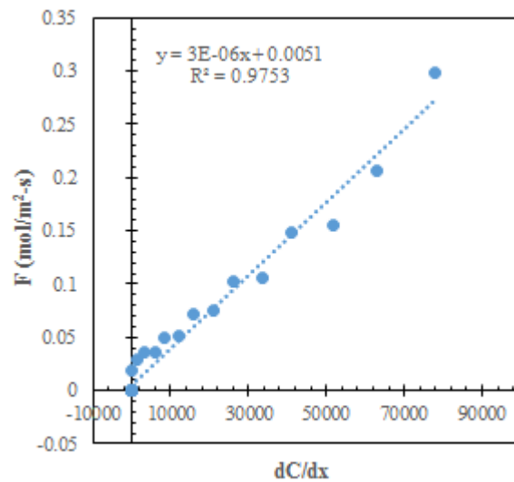
Figure 5. Soil \text{CO}_2 flux versus concentration gradient; VWC = 3.5%, replicate 1.
