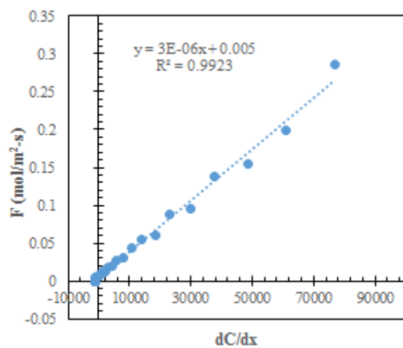
Figure 31. Soil CO 2 flux versus concentration gradient; VWC = 7.8%, replicate 10.
