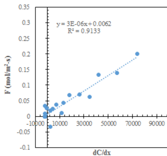
Figure 41. Soil CO 2 flux versus concentration gradient; VWC = 20.5%, replicate 10.
