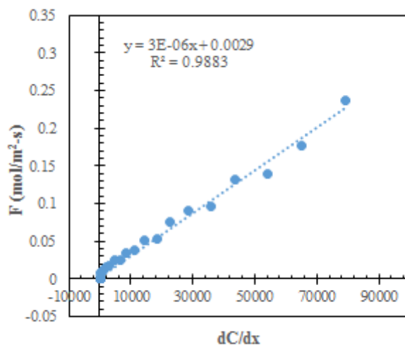
Figure 21. Soil CO 2 flux versus concentration gradient; VWC = 3.5%, replicate 10.
