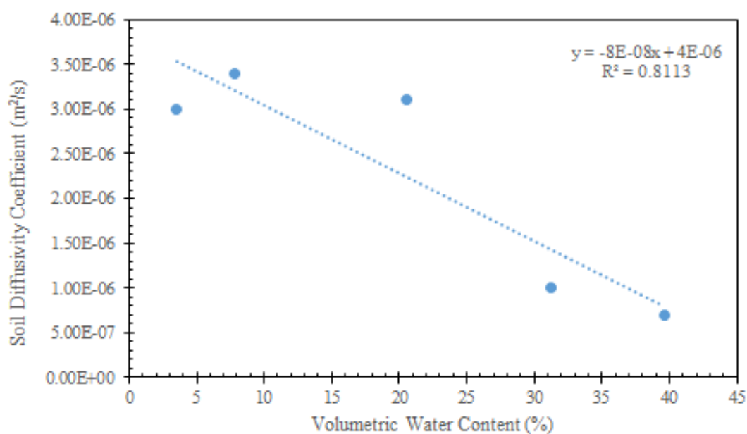
Figure 6. Fitted linear curve of soil volumetric water content versus soil diffusivity coefficients.
