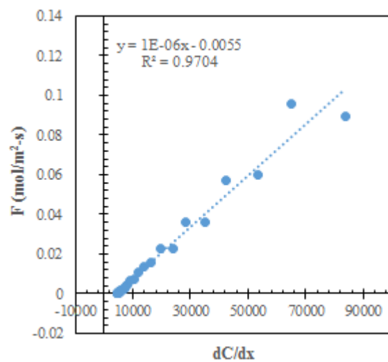
Figure 48. Soil CO 2 flux versus concentration gradient; VWC = 31.3%, replicate 7.
