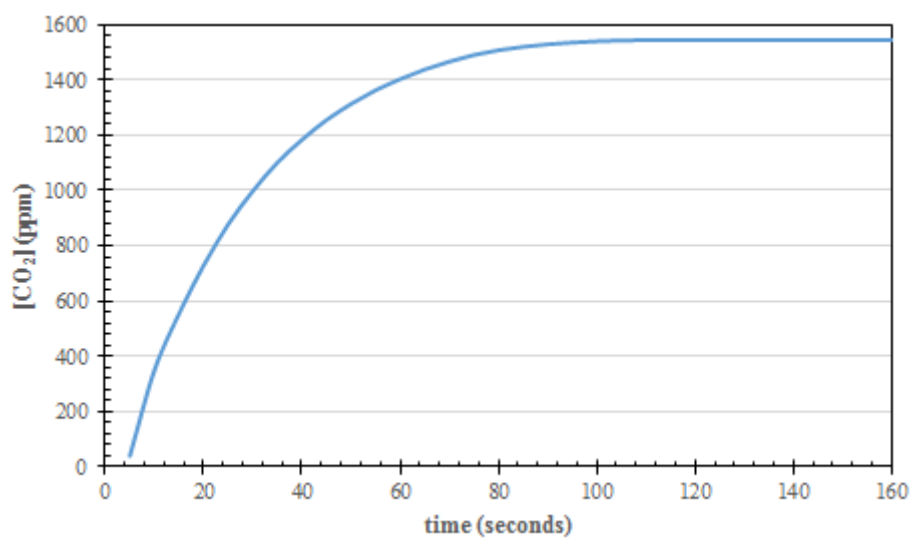
Figure 8. Soil CO 2 concentrations at VWC = 3.5%.
