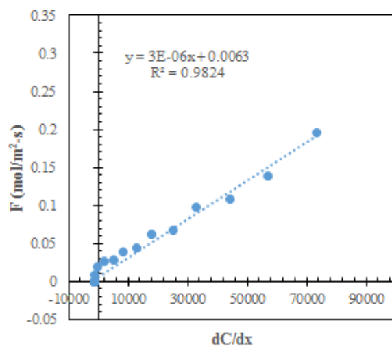
Figure 37. Soil CO 2 flux versus concentration gradient; VWC = 20.5%, replicate 6.
