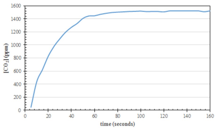
Figure 12. Soil CO 2 Concentrations at VWC = 39.6%.
