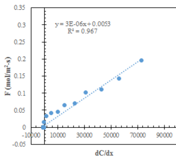
Figure 33. Soil CO 2 flux versus concentration gradient; VWC = 20.5%, replicate 2.
